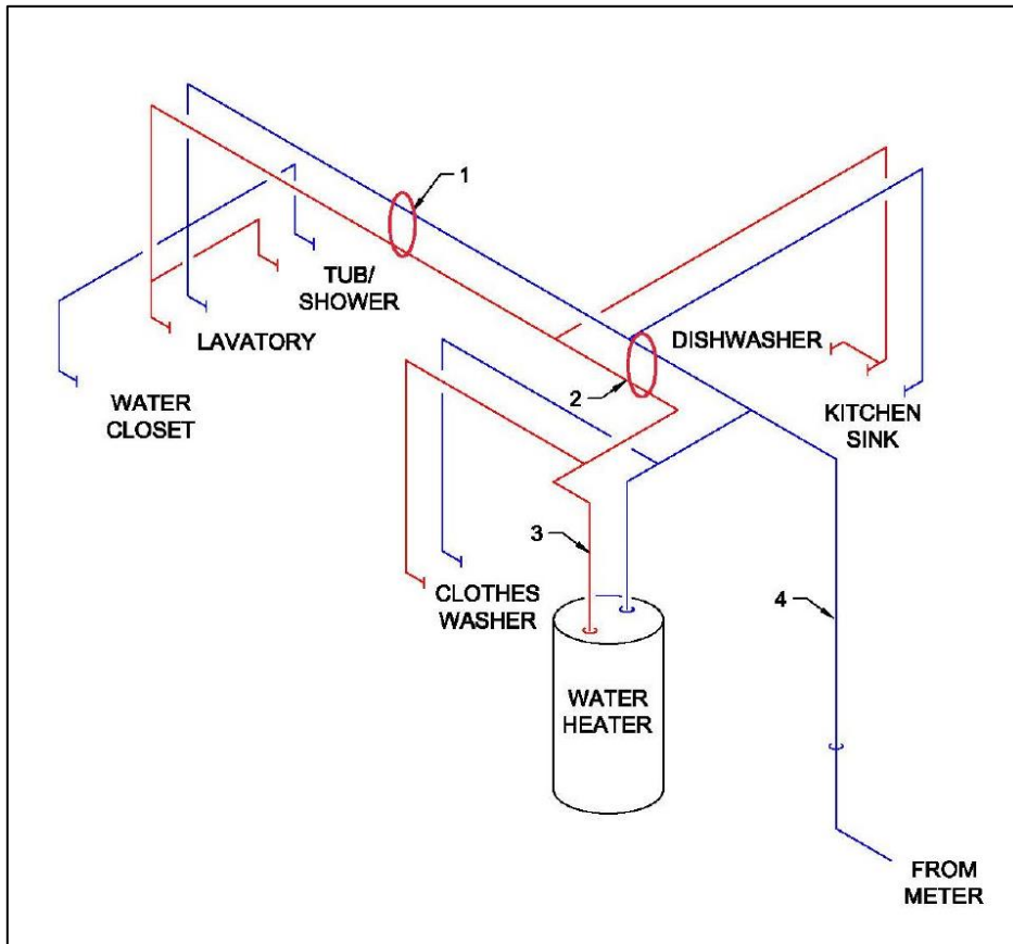
Figure 1 Isometric for Residential Home
